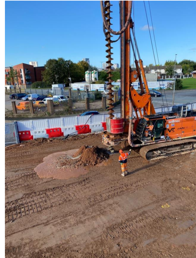
Rotary bored piling
