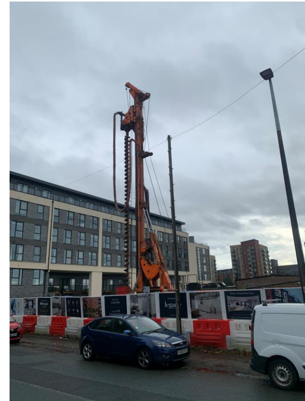
Ordsall Lane site view – Piling Rig
